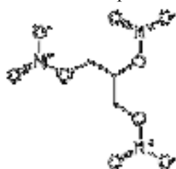
Tri Nitro Glycerol
