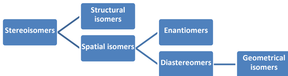
Figure : Classification of Stereoisomers
